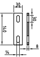
FISHPLATE
