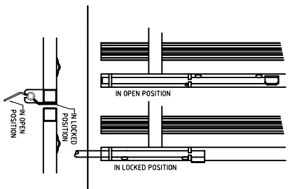
LOCK DETAIL scale 1/20
